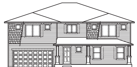
Elevation C
