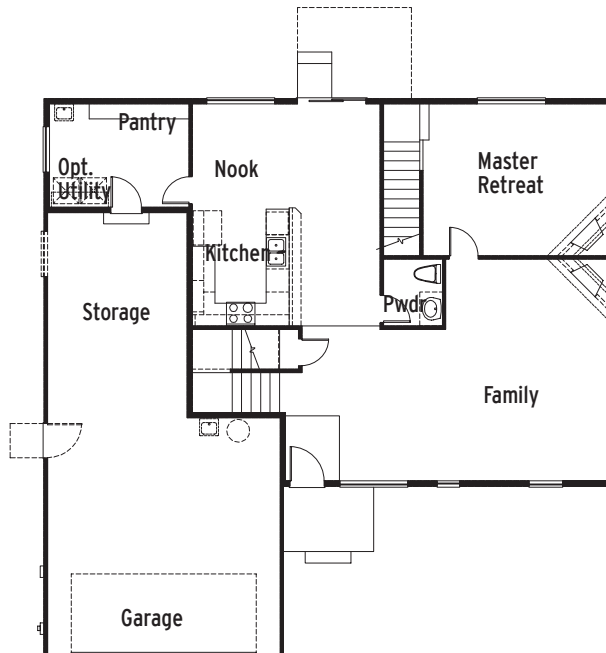
Plan 3441 Main Floor
