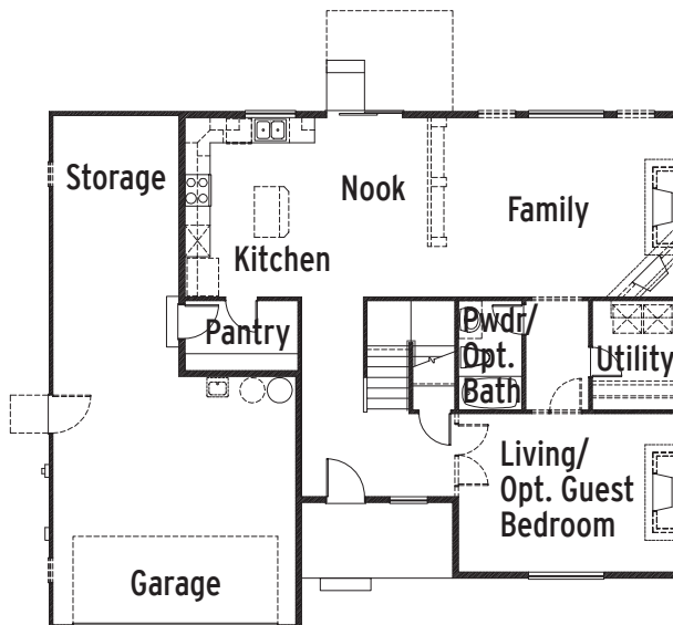
Plan 3241 Main Floor
