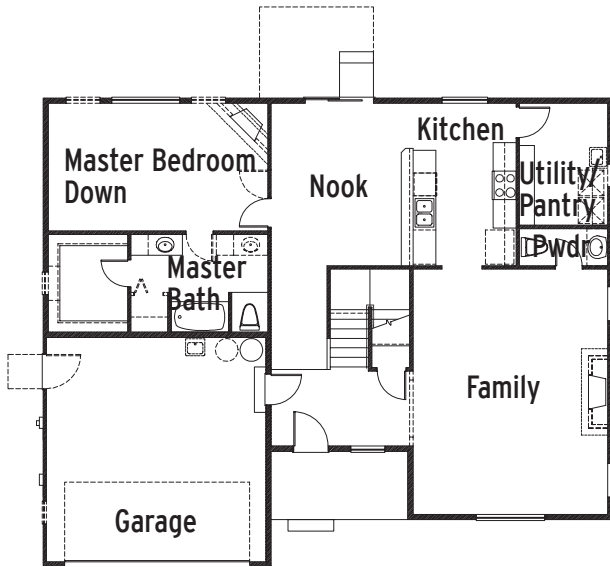
Plan 3231 Main Floor
