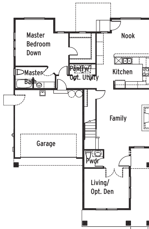
Plan 3142 Main Floor
