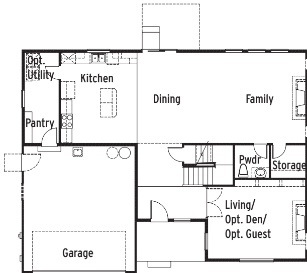
Plan 3155 Main Floor
