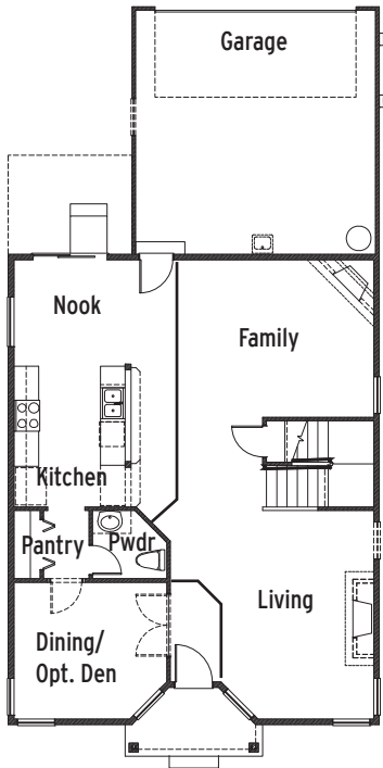
Plan 2655 Main Floor
