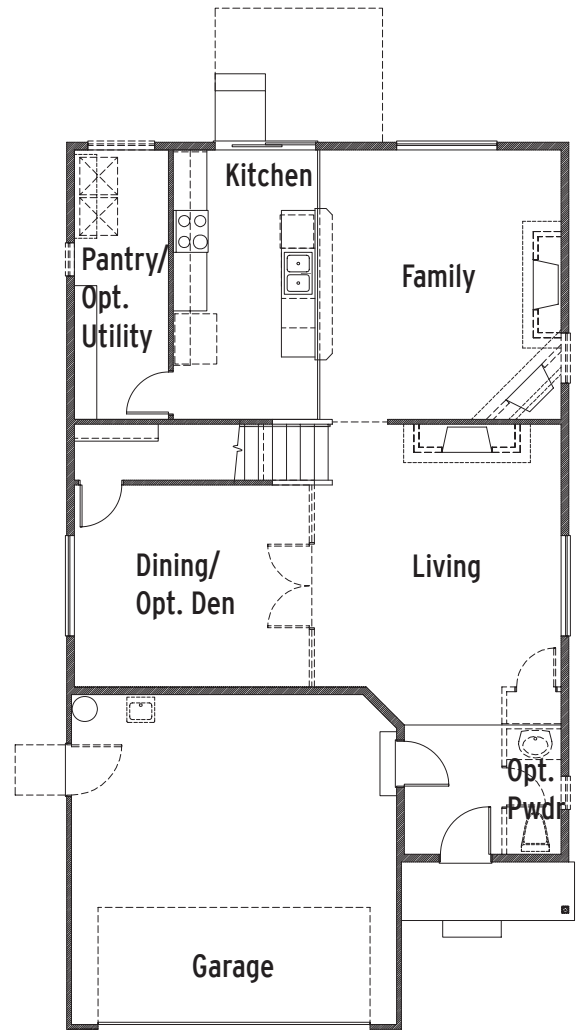
Plan 2565 Main Floor
