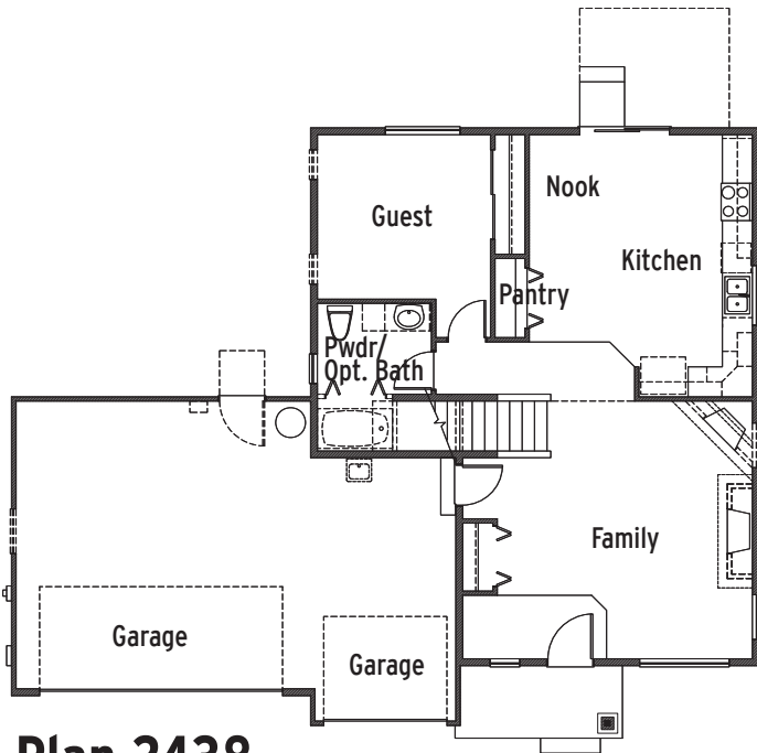
Plan 2438 Main Floor
