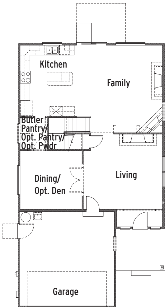
Plan 2413 Main Floor
