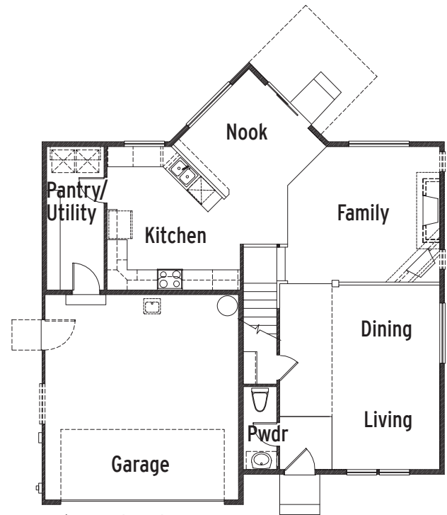
Plan 2421 Main Floor
