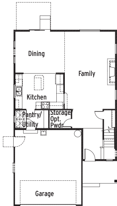
Plan 2313 Main Floor
