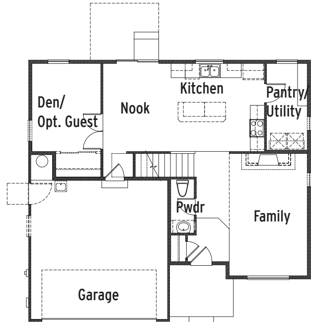
Plan 2265 Main Floor
