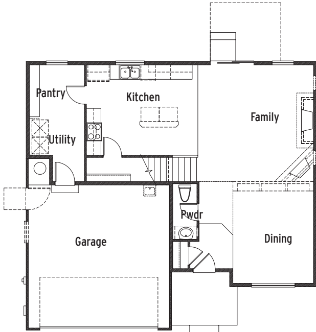
Plan 2255 Main Floor
