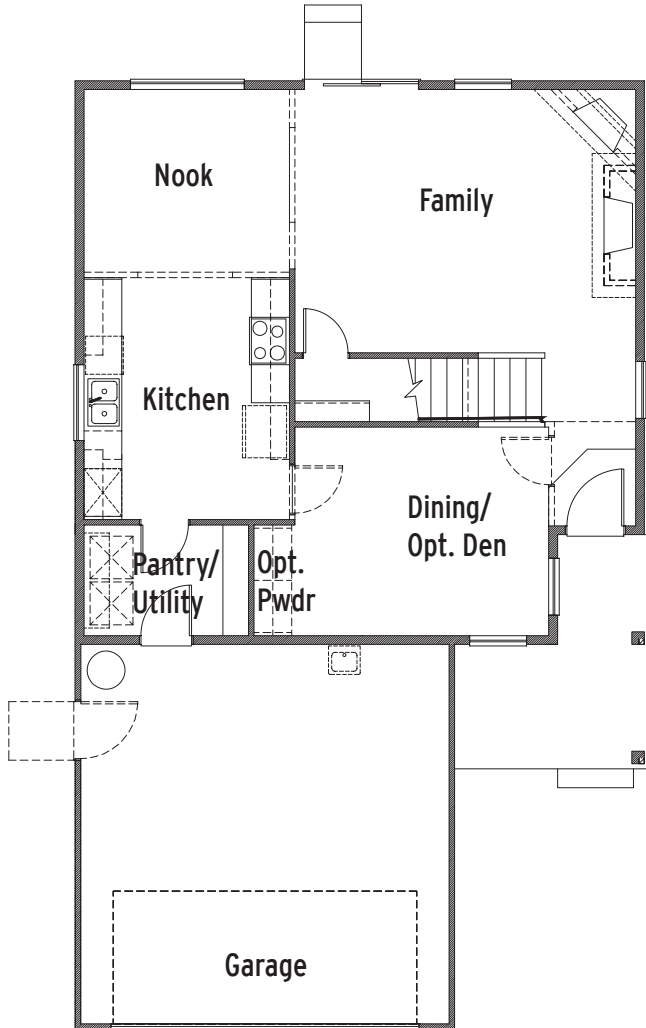
Plan 2111 Main Floor
