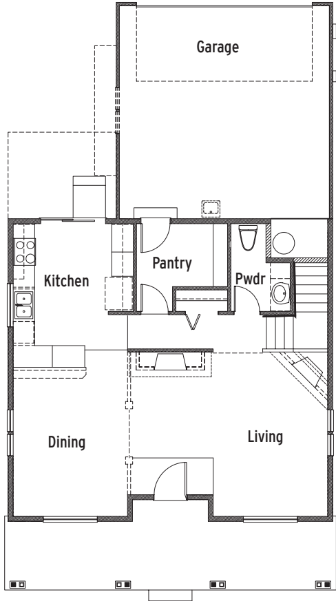
Plan 2015 Main Floor
