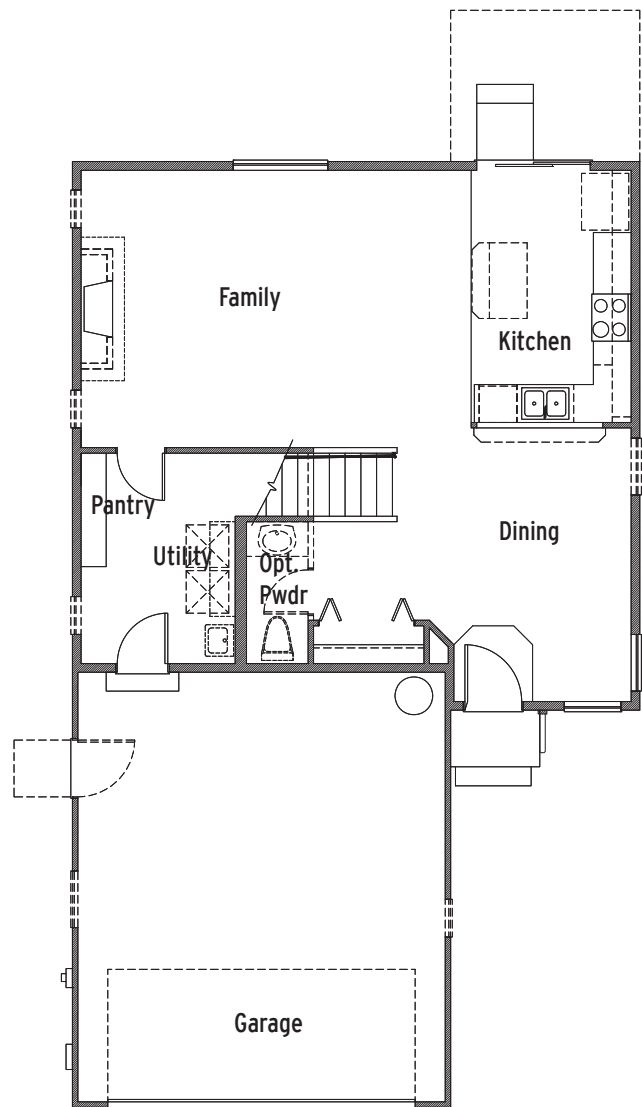
Plan 2002 Main Floor
