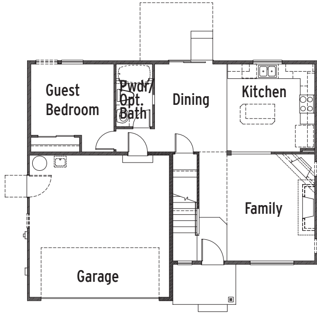
Plan 2075 Main Floor
