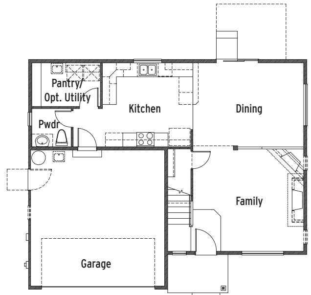
Plan 2065 Main Floor
