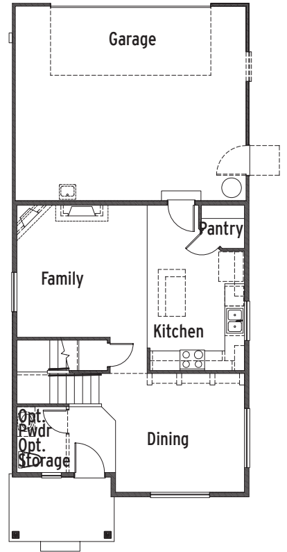
Plan 1836 Main Floor
