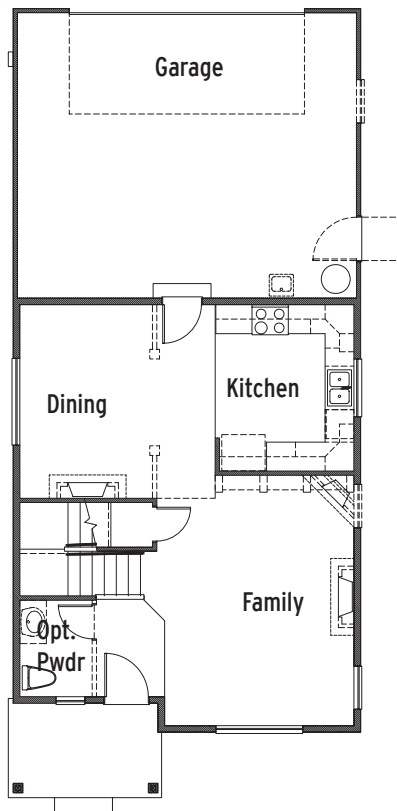
Plan 1826 Main Floor
