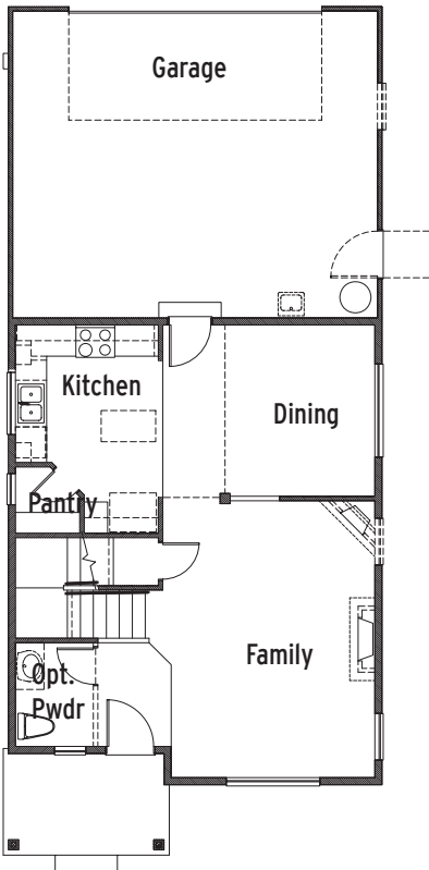
Plan 1816 Main Floor
