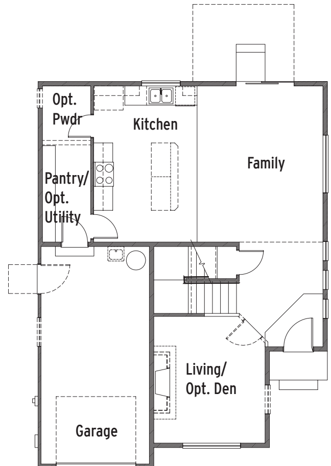
Plan 1865 Main Floor
