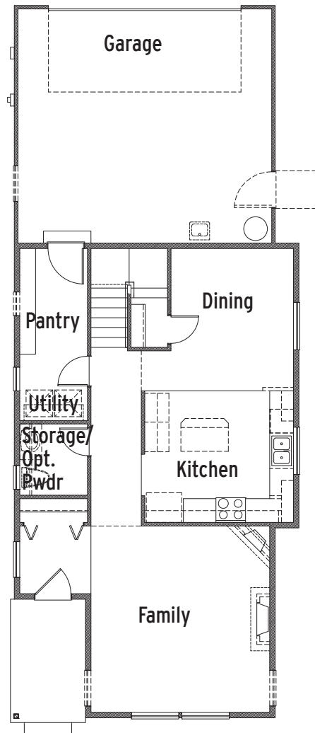
Plan 1722 Main Floor
