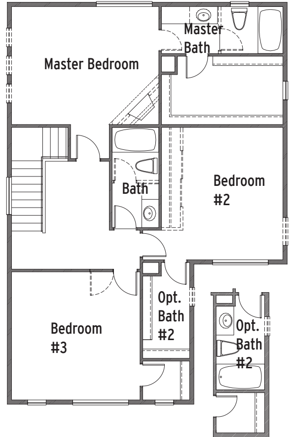
1700 Series Upper Floor
