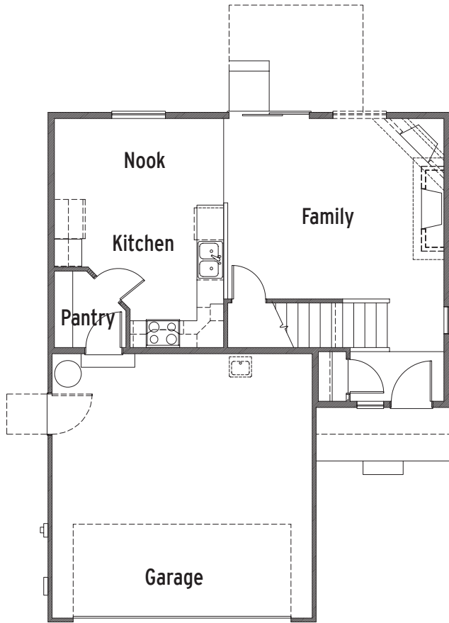
Plan 1531 Main Floor
