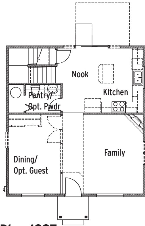
Plan 1227 Main Floor
