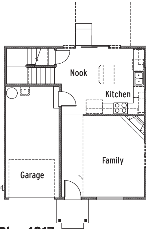
Plan 1217 Main Floor
