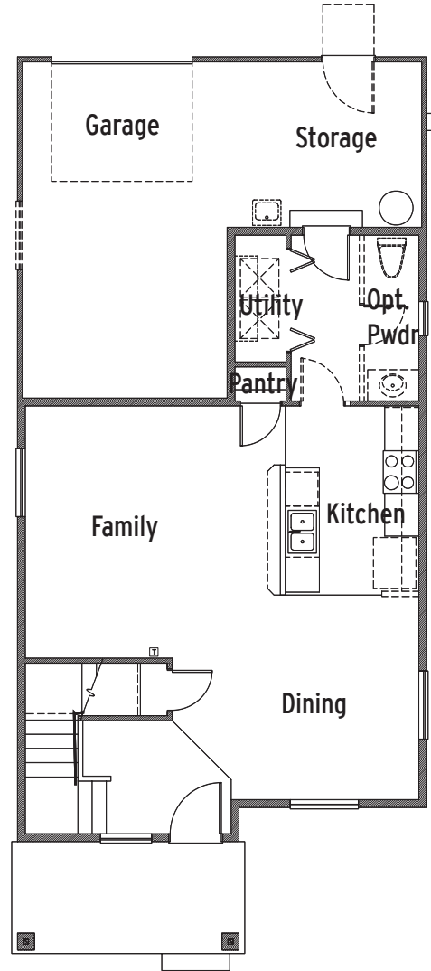
Plan 1222 Main Floor
