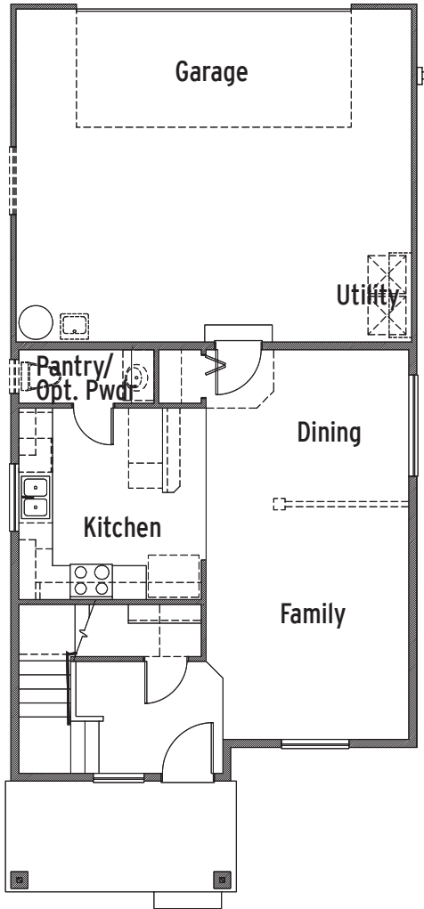
Plan 1212 Main Floor
