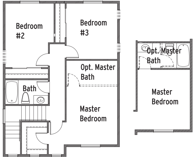
1220 Series Upper Floor
