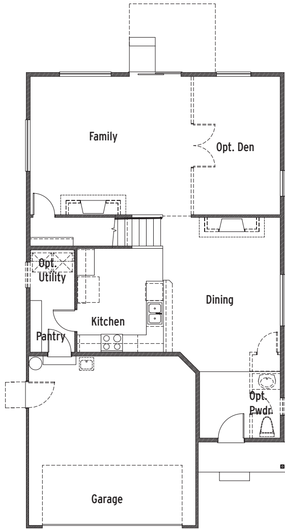
Plan 2555 Main Floor
