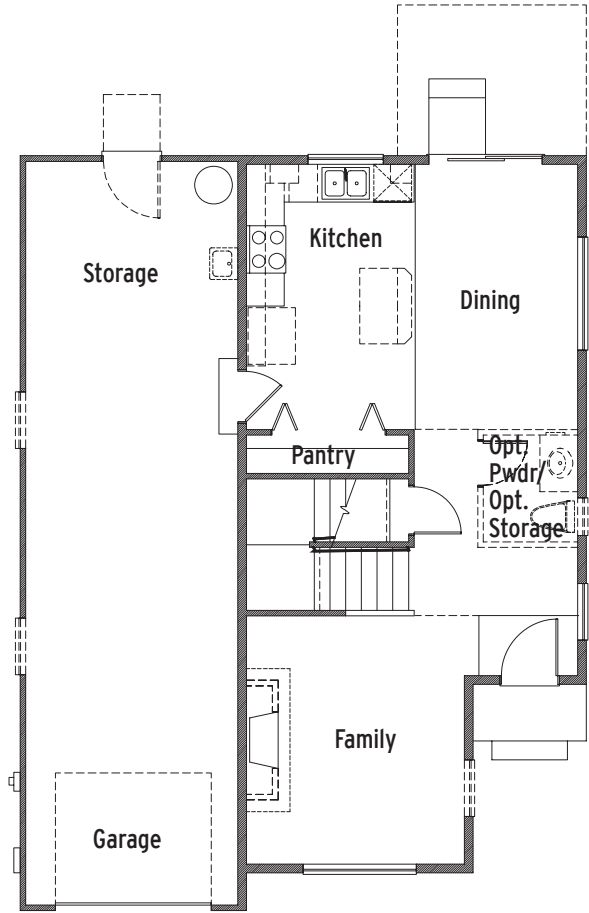
Plan 1665 Main Floor
