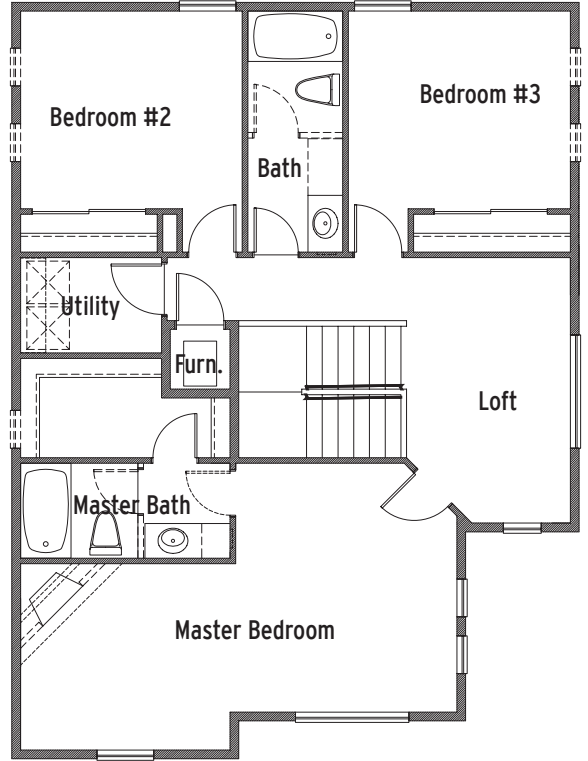
1650 Series Upper Floor
