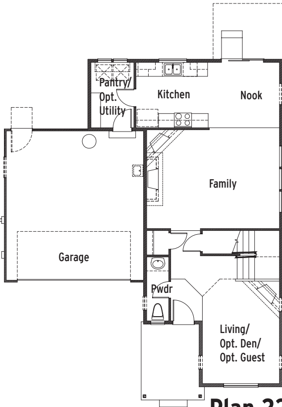
Plan 2244 Main Floor
